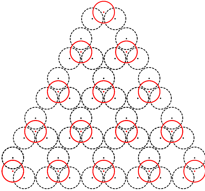
O-type + A-type
