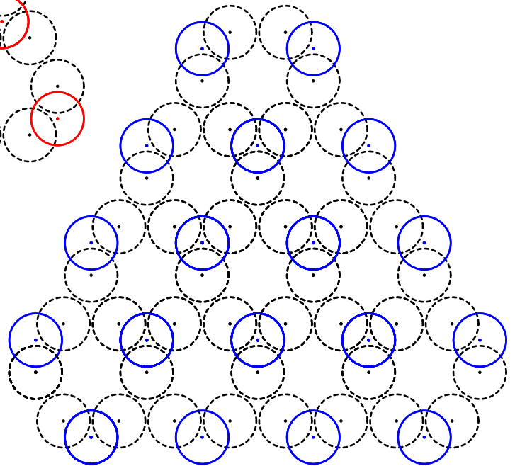
O-type + B-type
